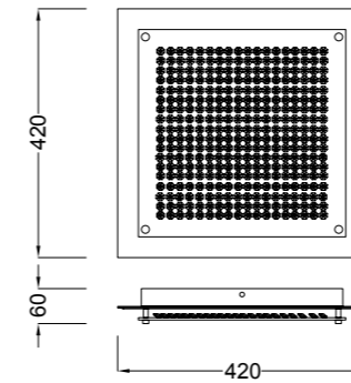
4582 - Plafón/Ceiling Lamp
