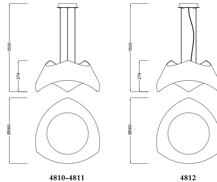
4810/4811/4812 - Colgante/Pendant Lamp
