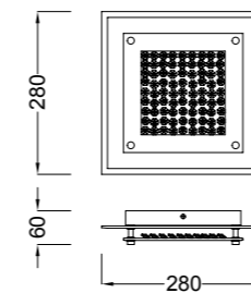
4580 - Plafón/Ceiling Lamp
