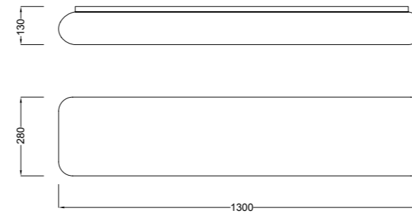
4671 - Plafón/Ceiling Lamp
